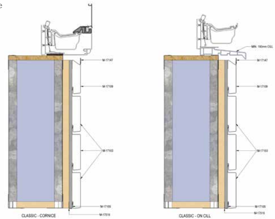
Classic with Facade
