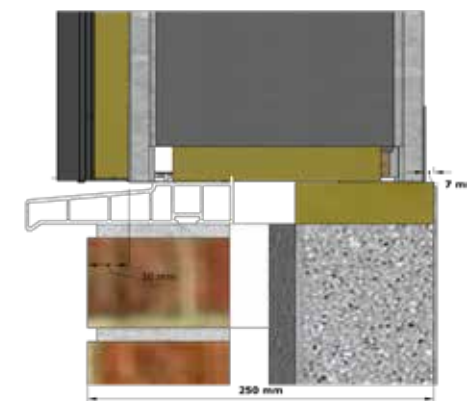
hup! on 250mm existing wall - on cill
